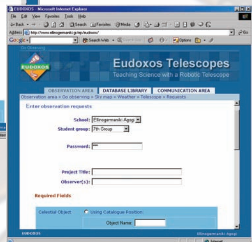
Figure 2.23: Password field
