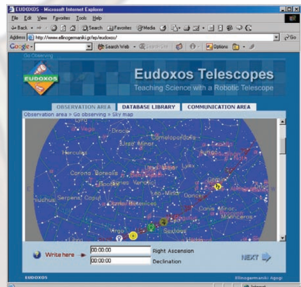
Figure 2.14: Sky map above the Eudoxos observatory
