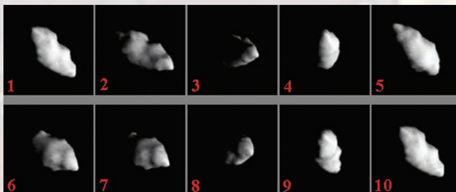
Figure 3.8: A sequence of views from Earth of asteroid Geographos that demonstrates how the cross-section varies with time.
