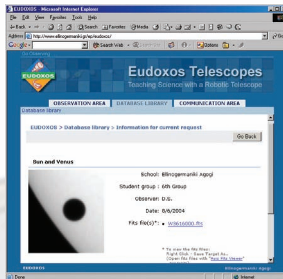
Figure 2.37: Image's info
