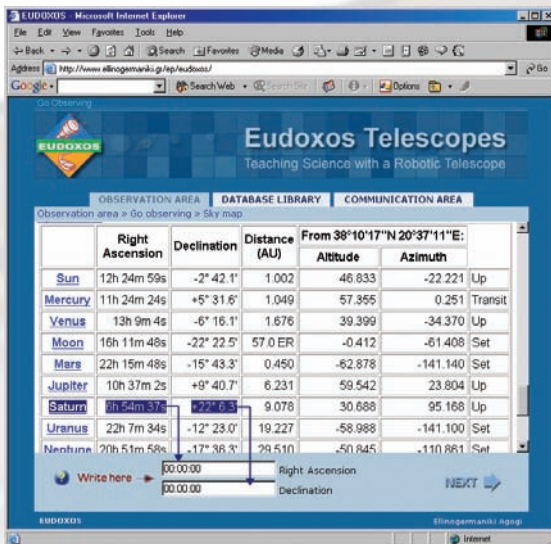
Figure 2.17: Right Ascension and Declination
