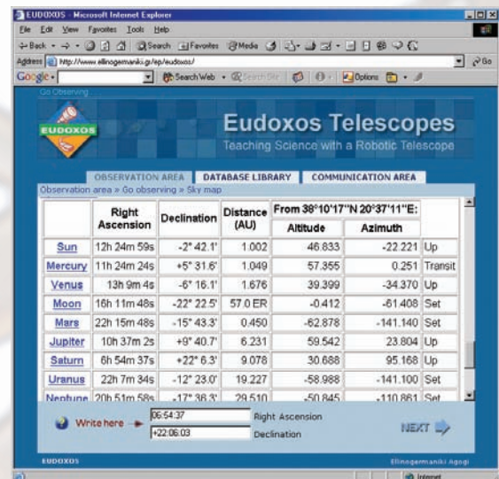
Figure 2.18: Appearance of astronomical object
