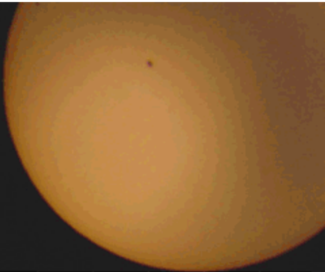
Observing the sun Rotation
